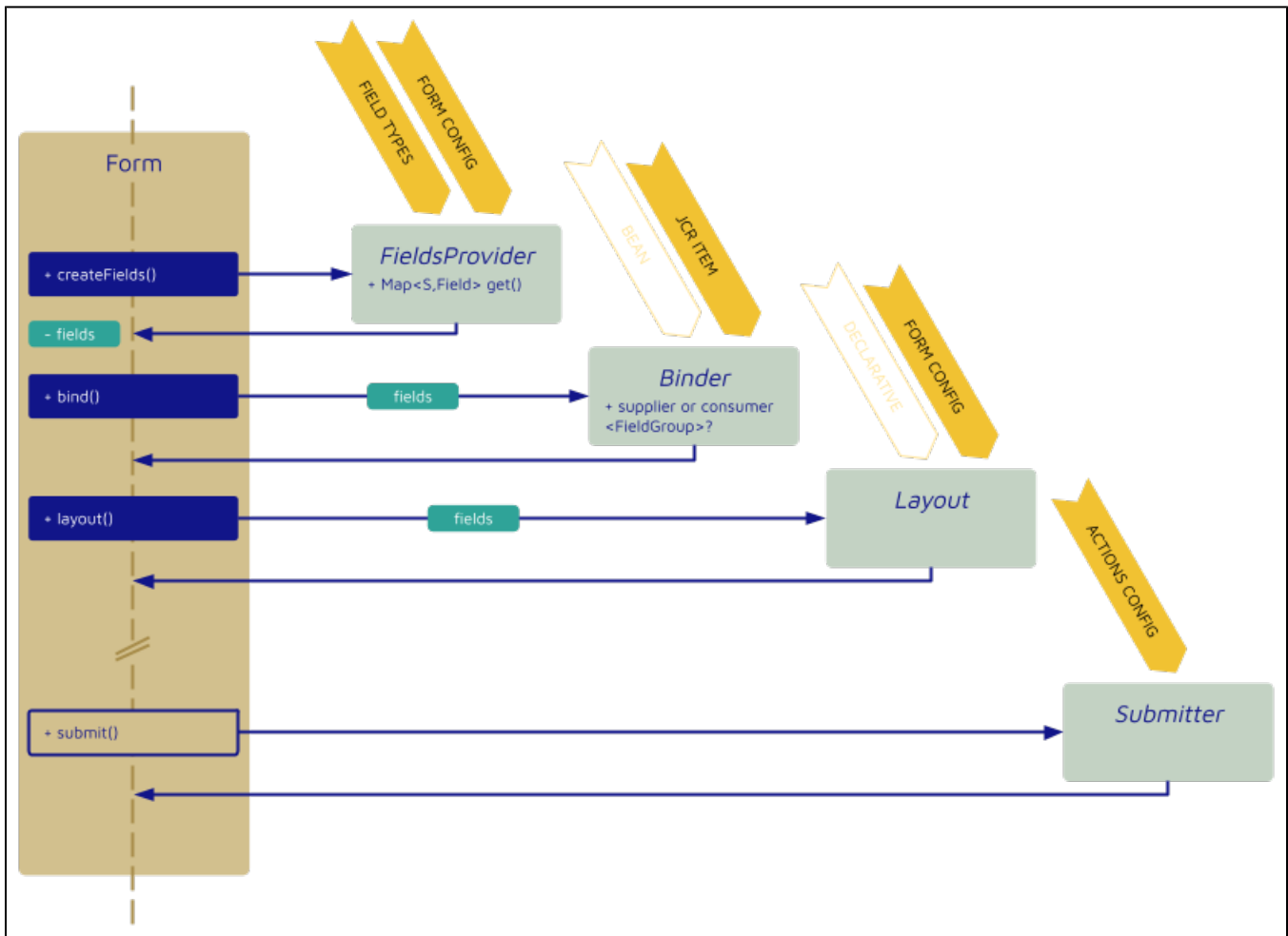
The Form component
